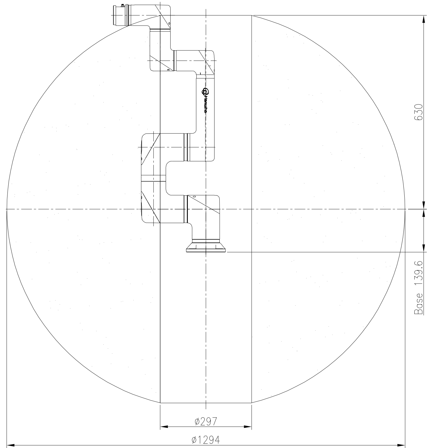
Working area, side view
